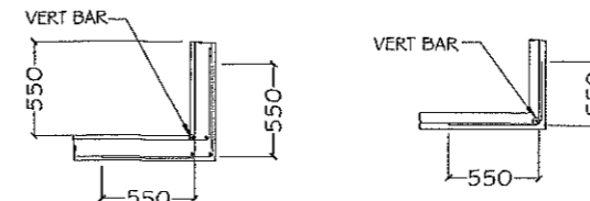
TYP. CONNECTION OF WALL @ CORNER
