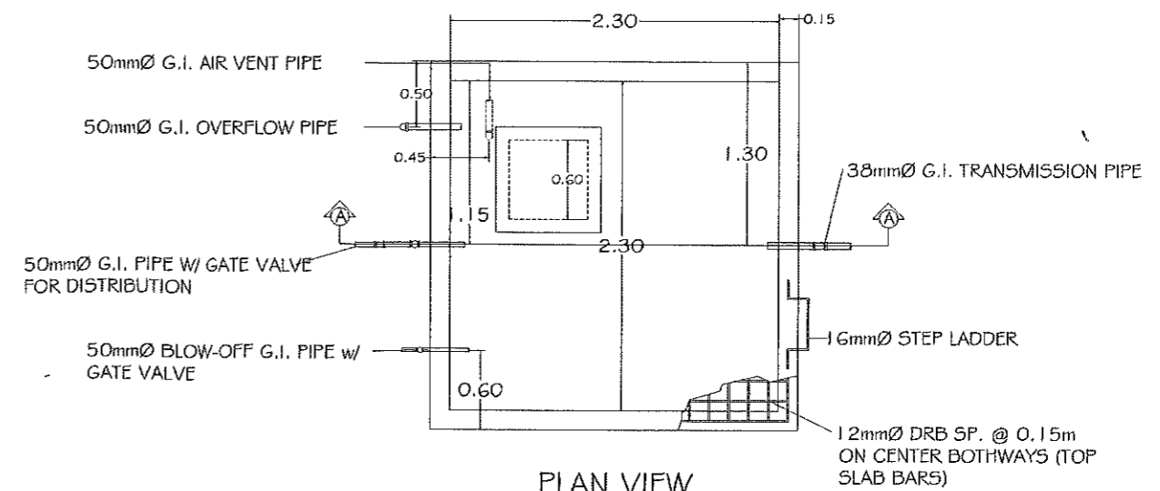
○ DETAILS OF RESERVOIR SCALE 1:20m
