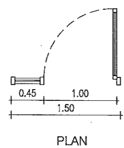
D1 PANEL DOOR W/ COMPLETE ACCESS & FITTINGS 1-SET D2 6MM THK. BRONZE GLASS DOOR, ANALOK FRAME 1-SET
