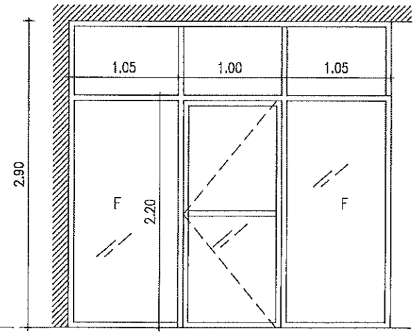
G1 6MM THK. BRONZE GLASS DOOR PARTITION, ANALOK FRAME 2-SETS
