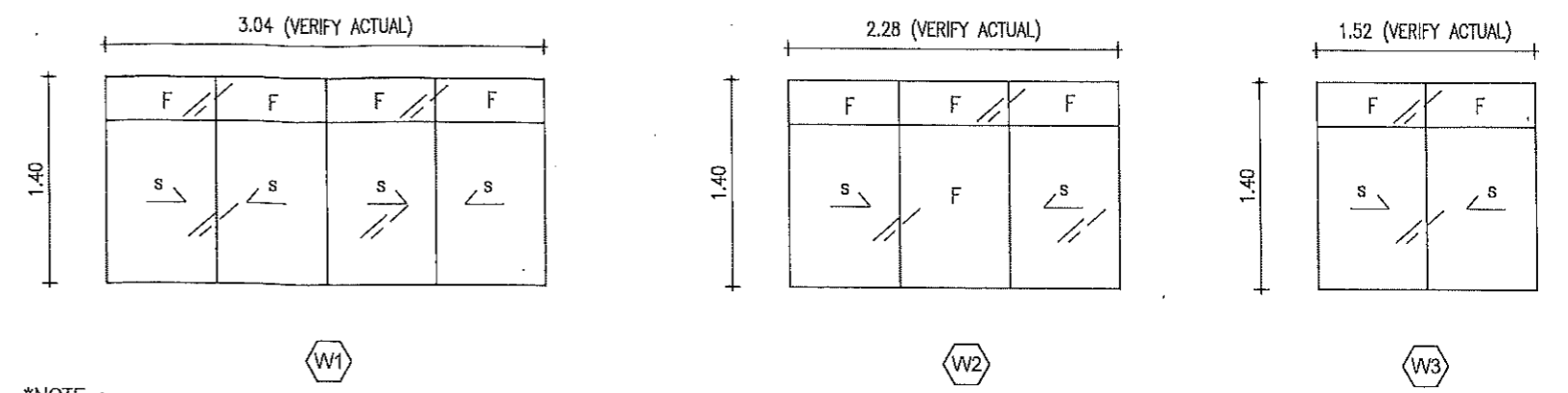
W1 6MM THK. BRONZE GLASS WINDOW, SLIDING TYPE, ANALOK FRAME 6-SETS W2 6MM THK. BRONZE GLASS WINDOW, SLIDING TYPE, ANALOK FRAME 6-SETS W3 6MM THK. BRONZE GLASS WINDOW, SLIDING TYPE, ANALOK FRAME 1-SET
