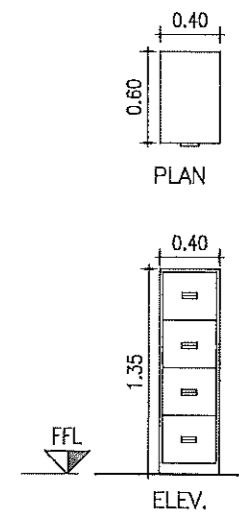
ELEV. 6-UNITS
