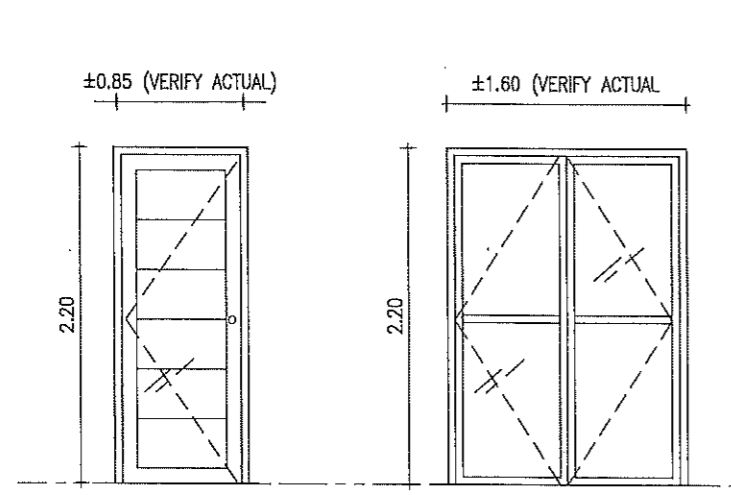
D1 PANEL DOOR W/ COMPLETE ACCESS & FITTINGS 1-SET D2 6MM THK. BRONZE GLASS DOOR, ANALOK FRAME 1-SET
