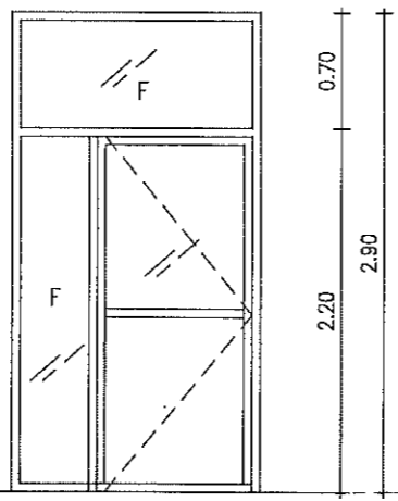
G2 6MM THK. BRONZE FIXED GLASS PARTITION, ANALOK FRAME 1-SET
