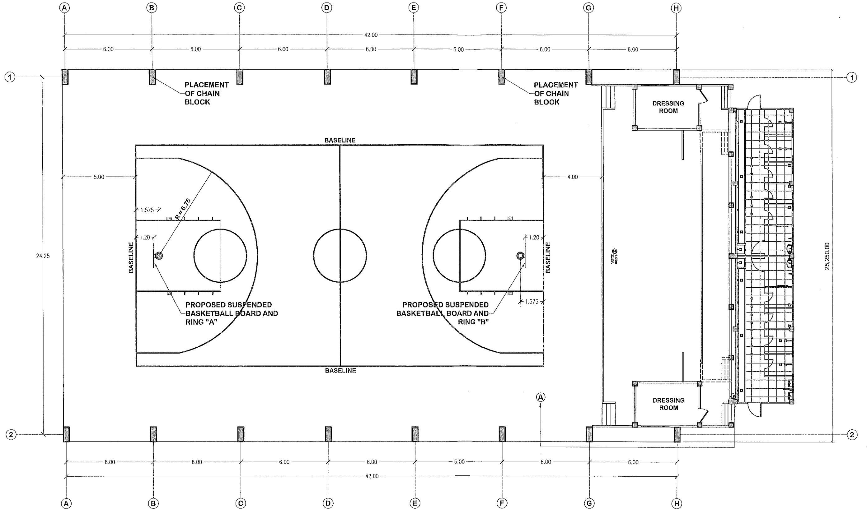
1 EXISTING FLOOR PLAN A-2 SCALE N T S
