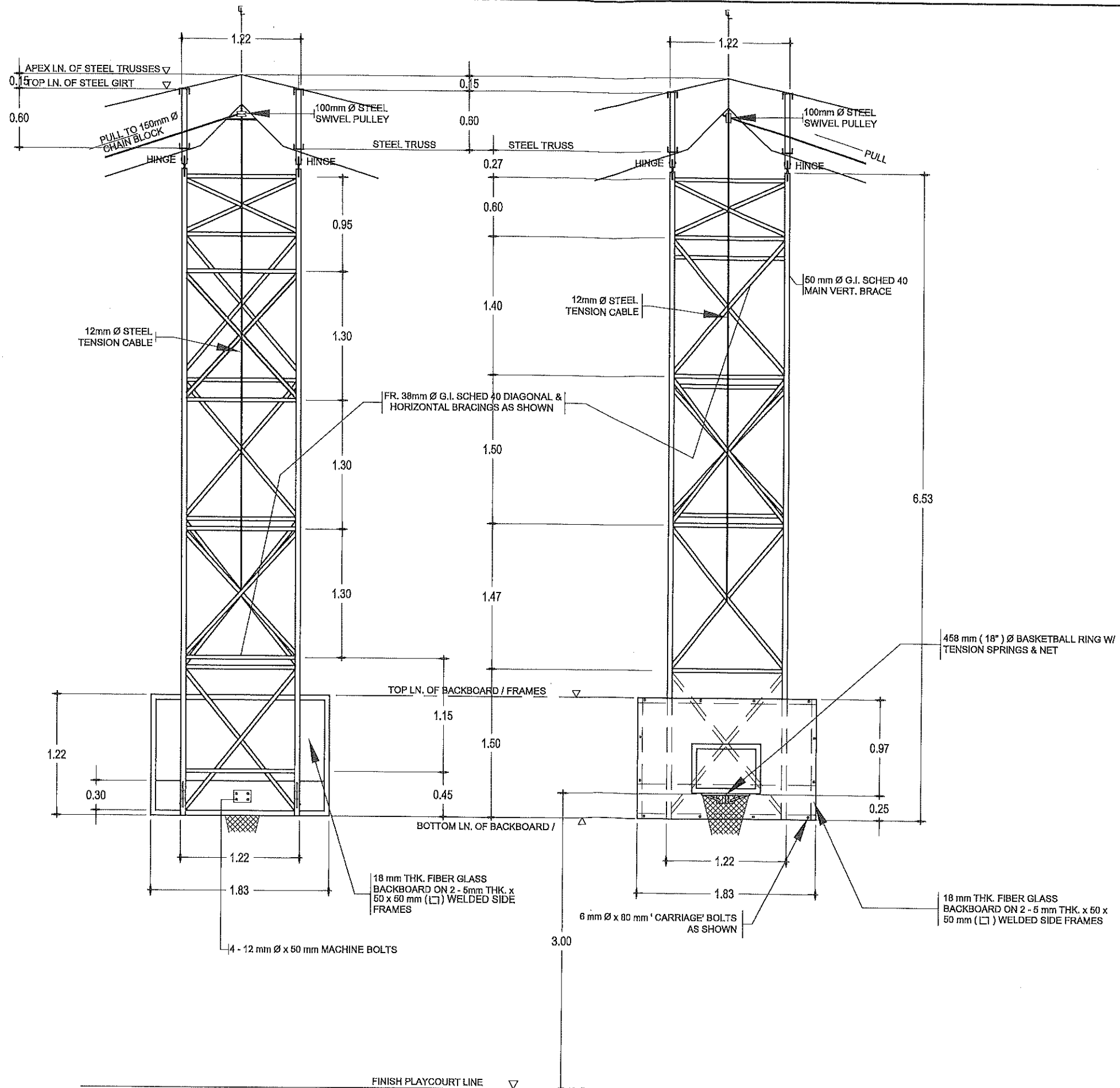
1 S-3 DETAIL OF SUSPENDED BASKETBALL BOARD & RING SCALE N T S
