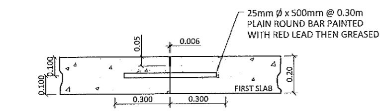
BUTT TRANSVERSE CONSTRUCTION OR CONTRACT JOINT
