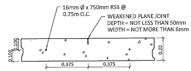
WEAKENED PLANE JOINT
