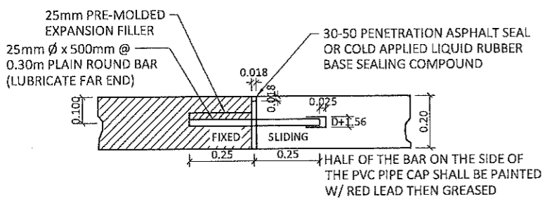
TYPICAL EXPANSION JOINT
