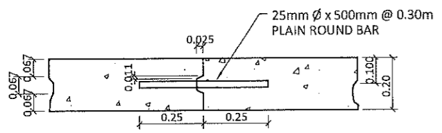
KEYED TRANSVERSE CONST. JOINT
