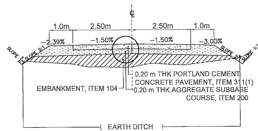
TYPICAL THRU FILL SECTION
