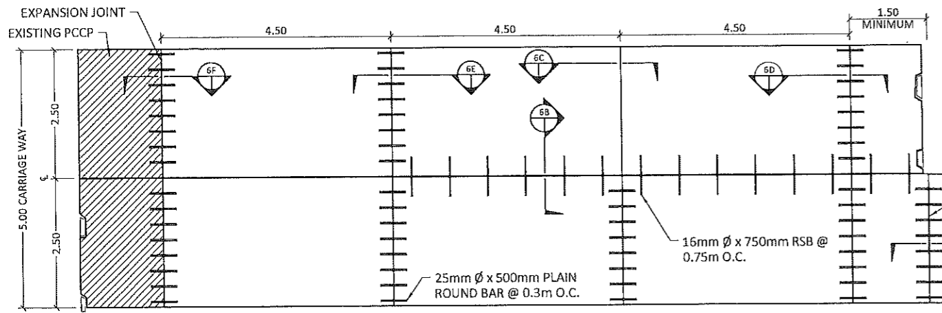
TYPICAL PLAN OF TWO-LANE PAVEMENT
