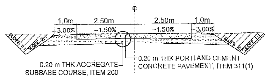
TYPICAL THRU CUT SECTION
