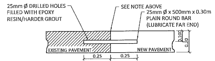
CONSTRUCTION JOINT
