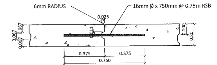
LONGITUDINAL CONST. JOINT
