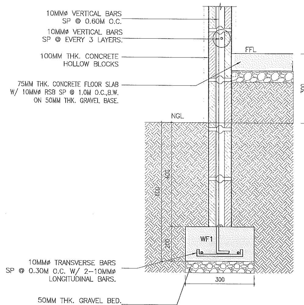
2 WF1 DETAIL S-3 SCALE 1:10 M.
