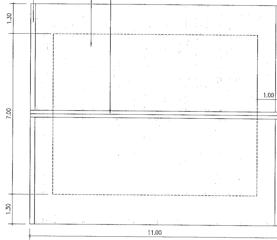
3 ROOF PLAN A-3 SCALE 1:100 M.
