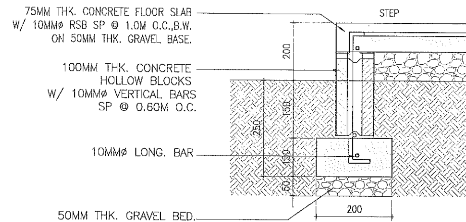
3 WF2 DETAIL S-3 SCALE 1:10 M.
