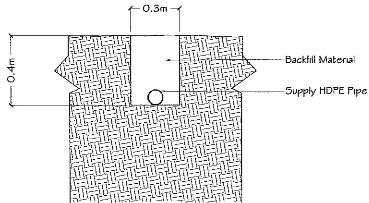
DETAIL OF PIPE LAYING SCALE NTS
