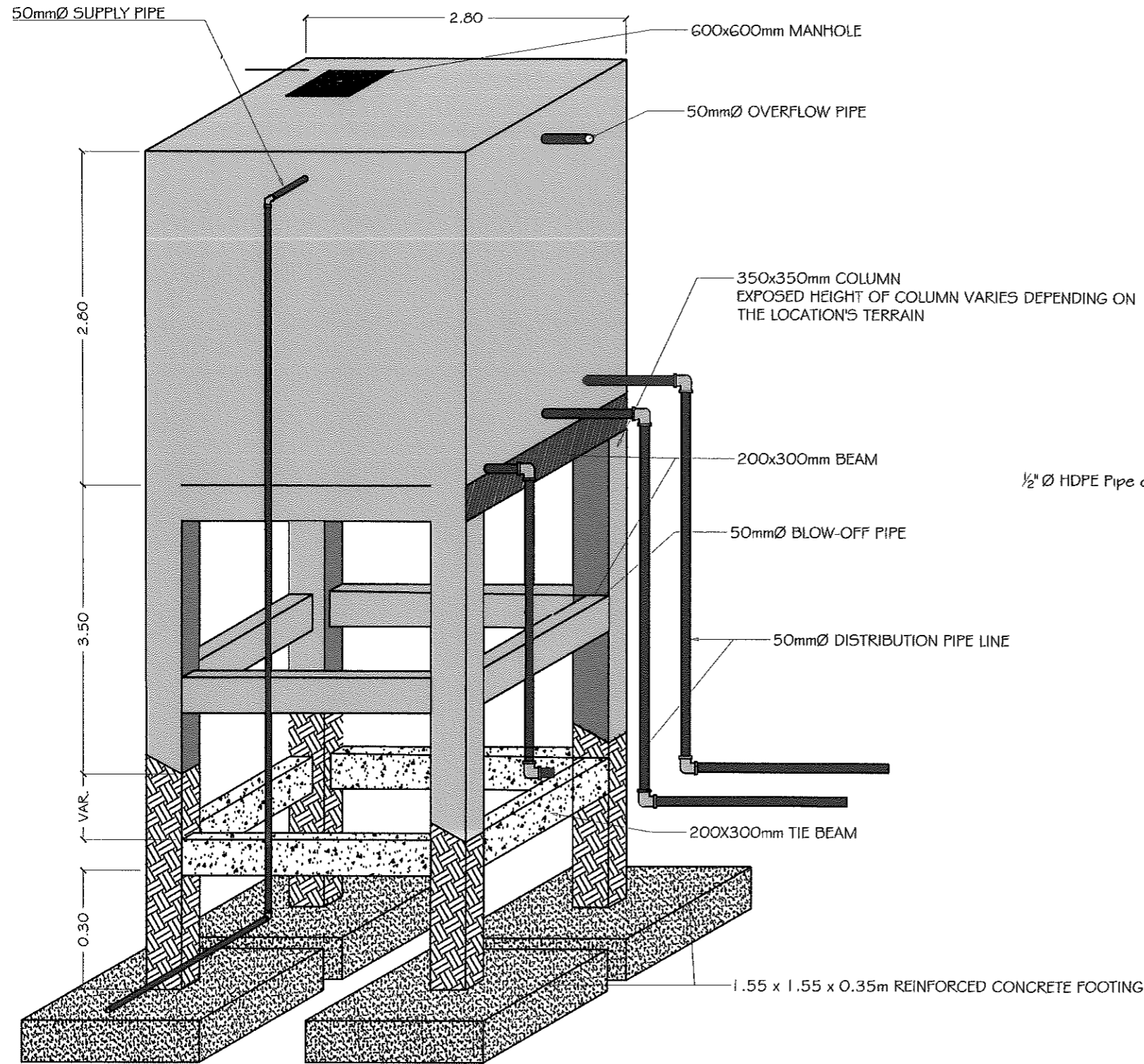
RESERVOIR ISOMETRIC VIEW SCALE NTS
