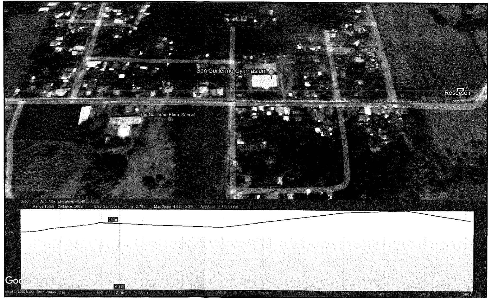
RESERVOIR TO DISTRIBUTION PROFILE
