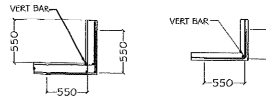
TYP. CONNECTION OF WALL @ CORNER
