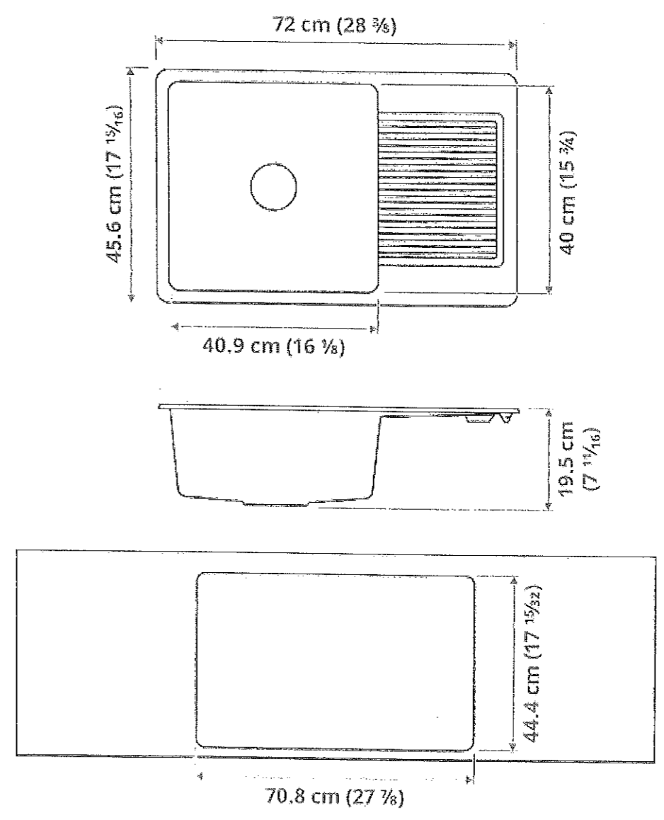
2 KITCHEN SINK DETAIL A-68
