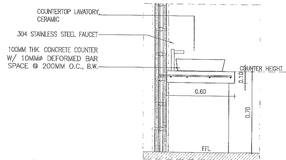
1 TYPICAL CONCRETE COUNTER DET. A-61 SCALE 1:20M.
