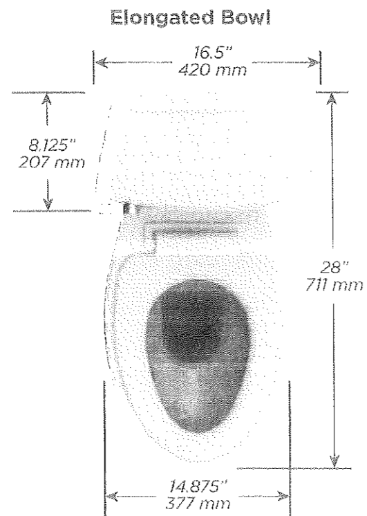
TYPICAL WATER CLOSET DET.
