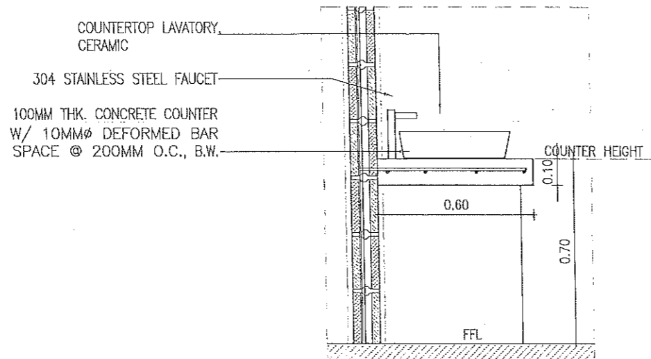
1 TYPICAL CONCRETE COUNTER DET. A-32 SCALE 1:20M.
