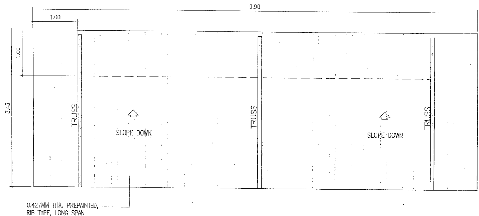
2 ROOF PLAN A-66 SCALE 1:50
