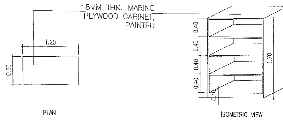
3 SHELVES DETAIL A-7 SCALE 1:50
