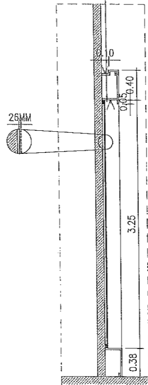
SECTION VIEW
