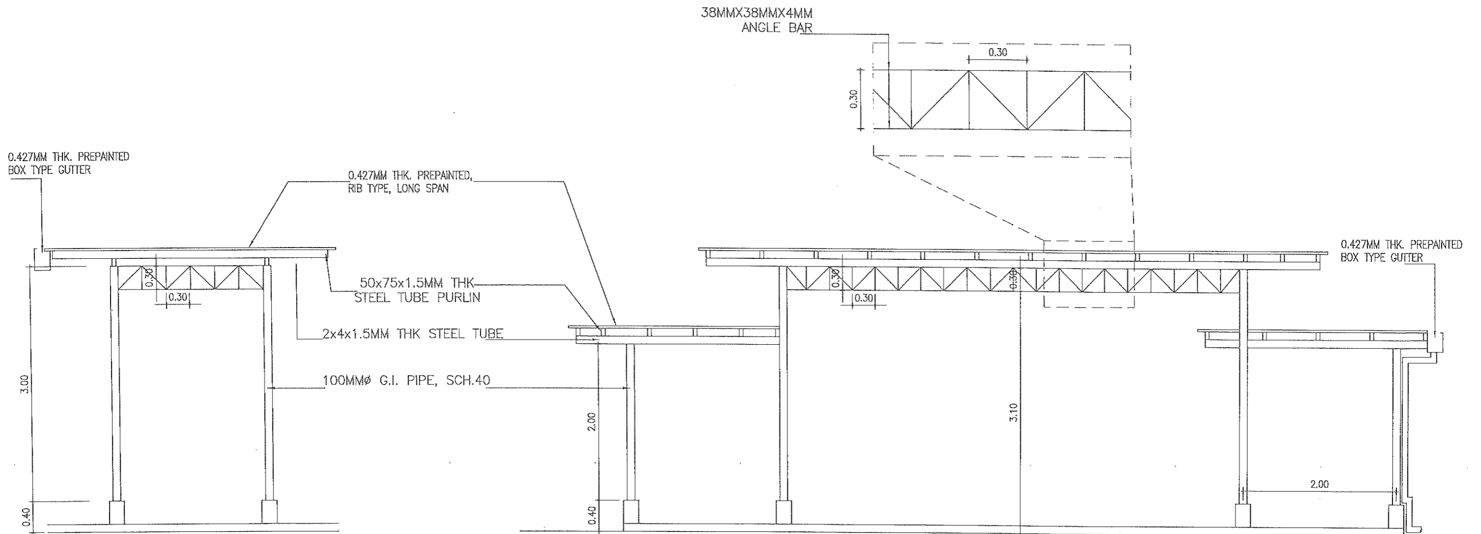
1 CROSS SECTION A-72 SCALE 1:20 M.
