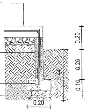
2 WALL FOOTING (WF-01) DET. A-8 SCALE 1:20
