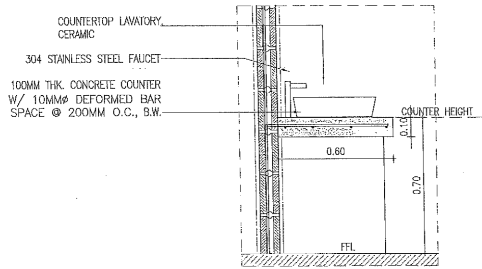
3 TYPICAL CONCRETE COUNTER DET. A-39 SCALE 1:20M.
