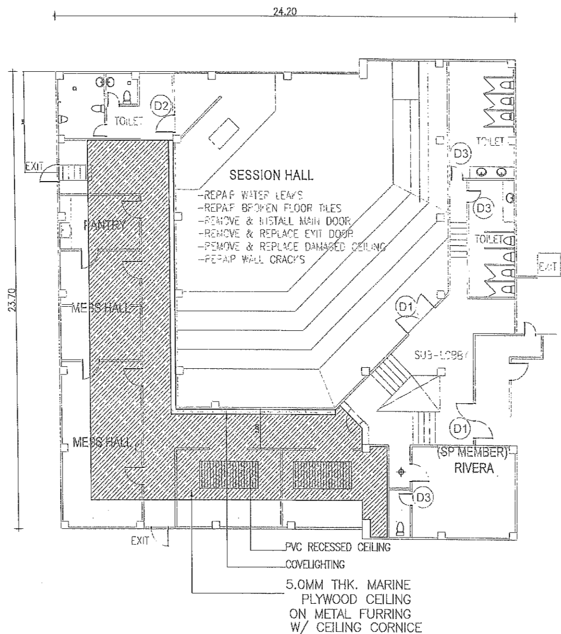
1 CEILING DETAIL A-21 SCALE 1:100
