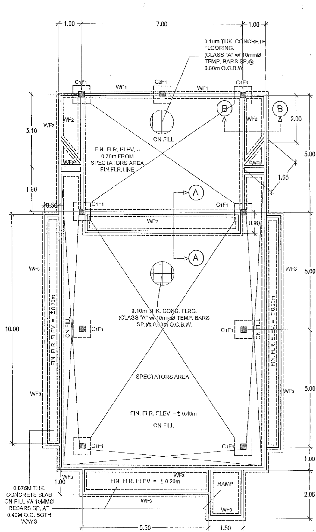
1 FOUNDATION PLAN SCALE 1:100
