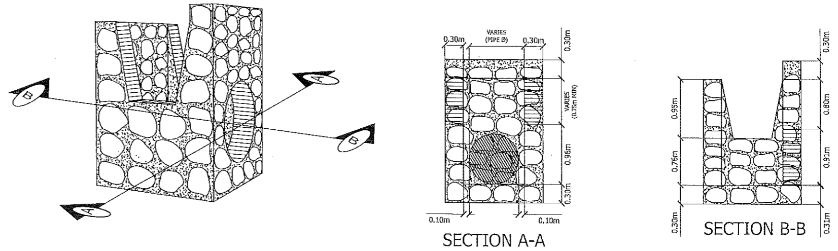
STONE MASONRY CATCH BASIN DETAIL SCALE DNTS
