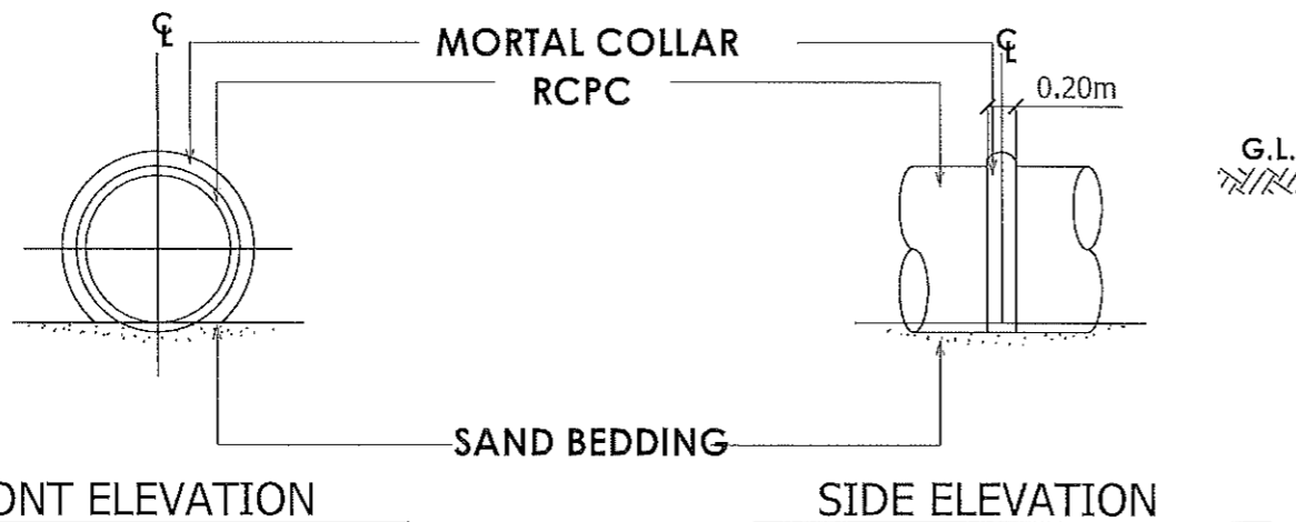
COLLAR DETAIL SCALE DNTS
