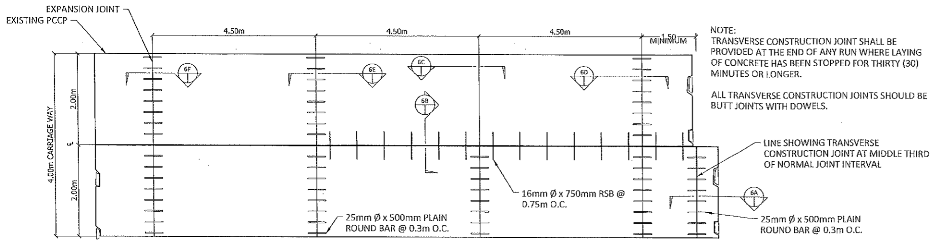
TYPICAL PLAN OF TWO-LANE PAVEMENT SCALE: 1:100m
