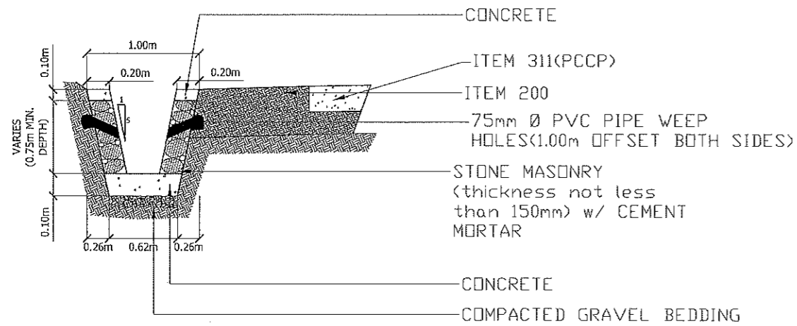
STONE MASONRY LINED CANAL DETAIL SCALE DNTS
