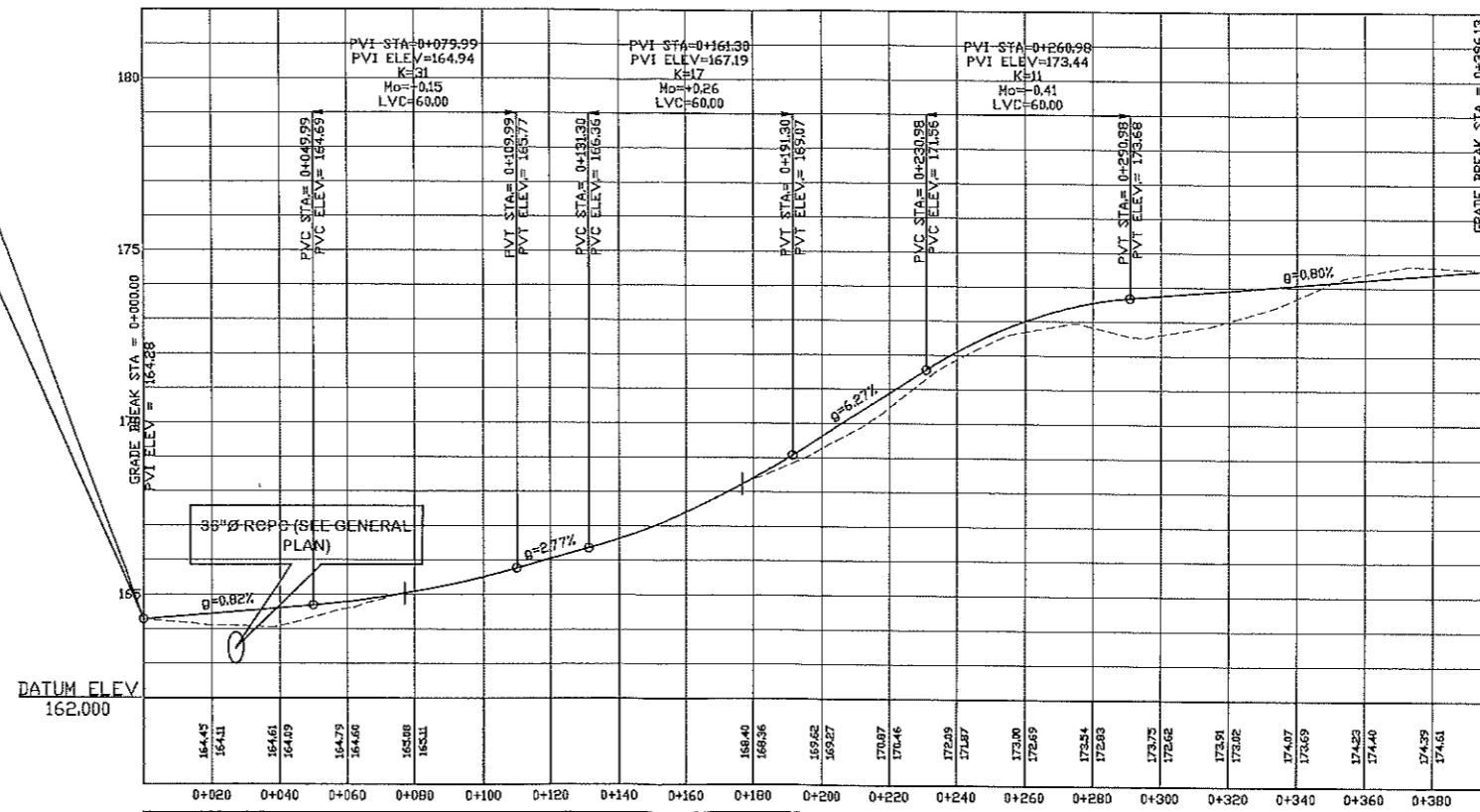
Vertical Curvature
