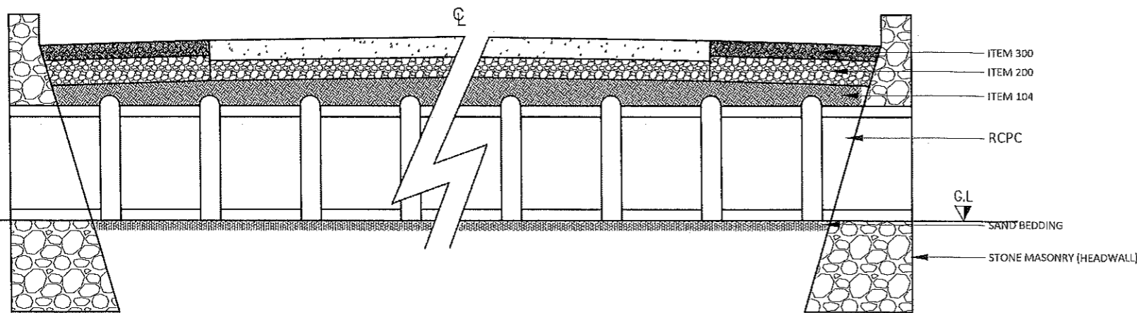
TYPICAL REINFORCED CONCRETE PIPE CULVERT SCALE DNTS
