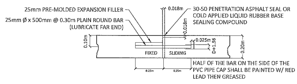
TYPICAL EXPANSION JOINT TO BE PLACED EVERY 36.00 M. O.C. SCALE: 1:20m
