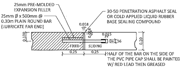
TYPICAL EXPANSION JOINT TO BE PLACED EVERY 36.00 M. O.C. SCALE: 1:20m
