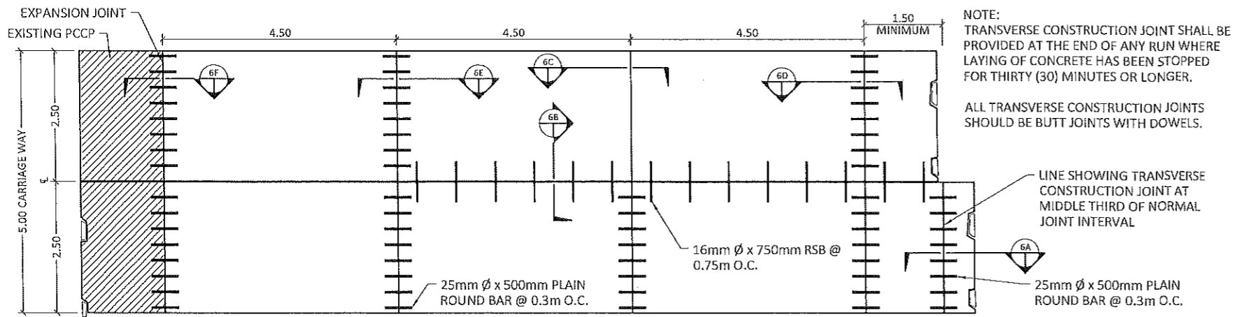
TYPICAL PLAN OF TWO-LANE PAVEMENT SCALE: 1:100m
