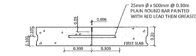
BUTT TRANSVERSE CONSTRUCTION OR CONTRACT JOINT SCALE: 1:20m
