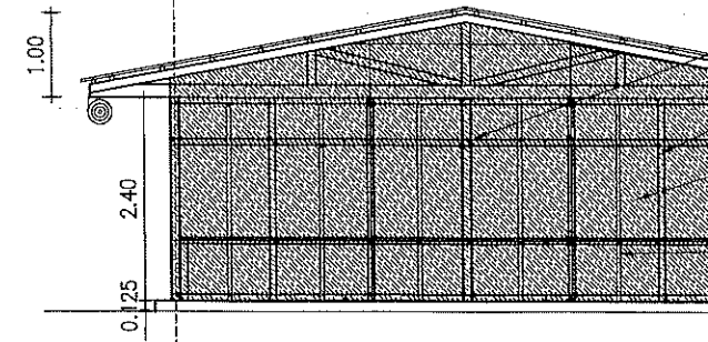
2 SECTION THRU "A-A" SCALE 1:100 M.
