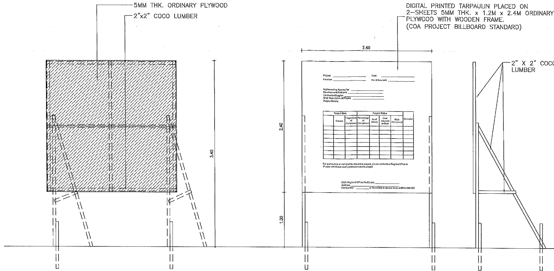
1 PROJECT BILLBOARD DETAIL 0-1 SCALE 1:40 M.
