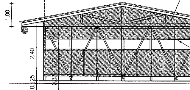
3 ELEVATION "B & C" SCALE 1:100 M.
