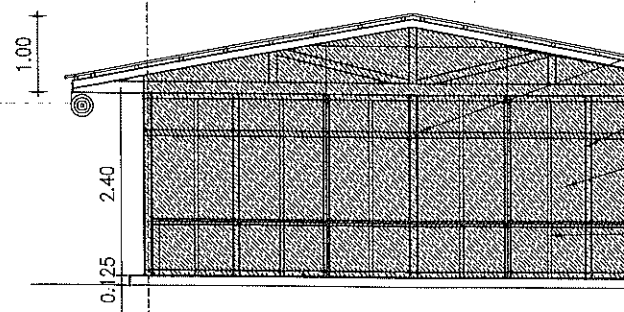
2 SECTION THRU "A-2" SCALE 1:100 M.
