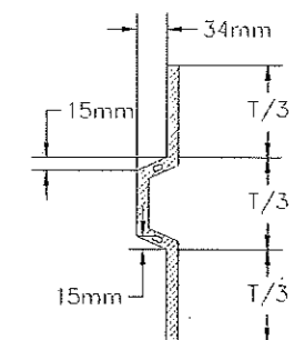
DETAIL OF SIDE FORMS NOT TO SCALE
