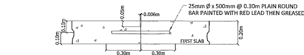
BUTT TRANSVERSE CONSTRUCTION OR CONTRACTION JOINT SCALE: 1:20m
