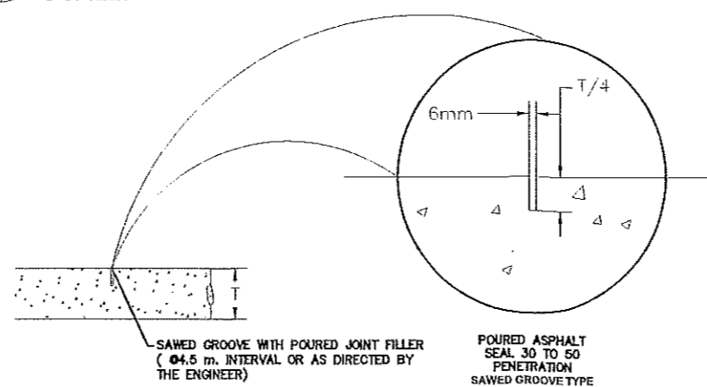
WEAKENED PLANE JOINT OR CONTRACTION JOINT NOT TO SCALE
