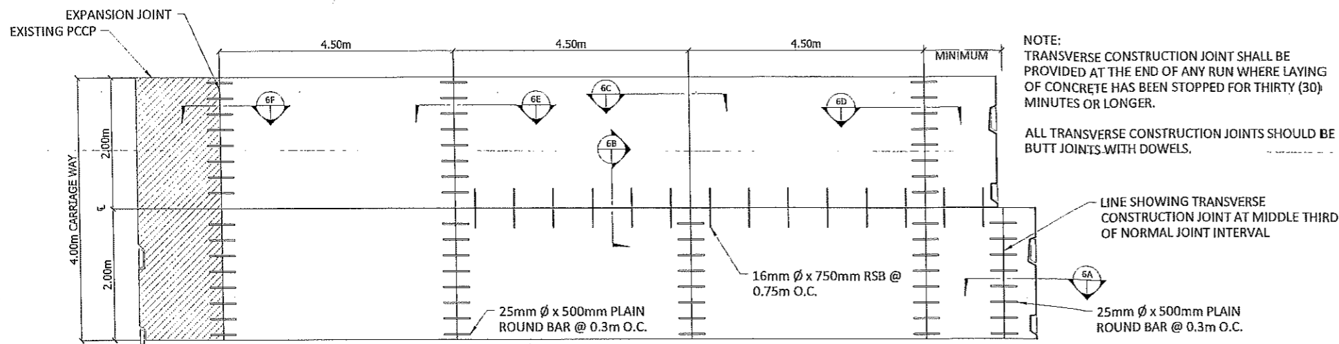
TYPICAL PLAN OF TWO-LANE PAVEMENT SCALE: 1:100m
