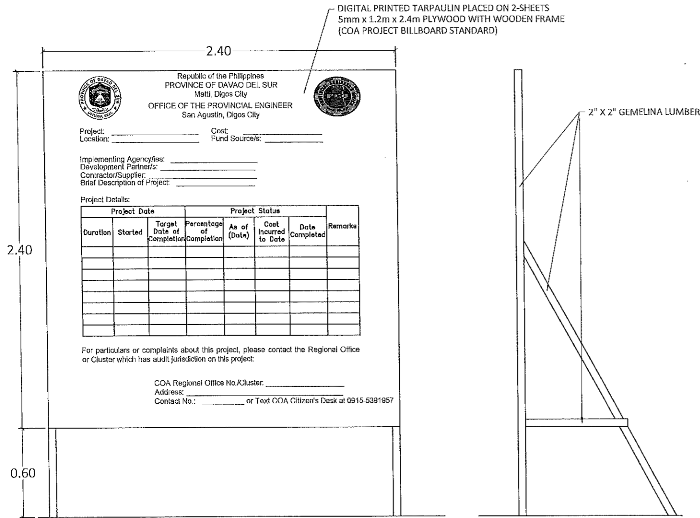
PROJECT BILLBOARD (COA STANDARDS) SCALE 1:25m
