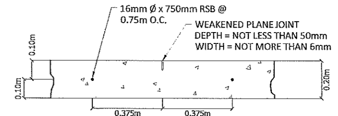
WEAKENED PLANE JOINT SCALE: 1:20m
