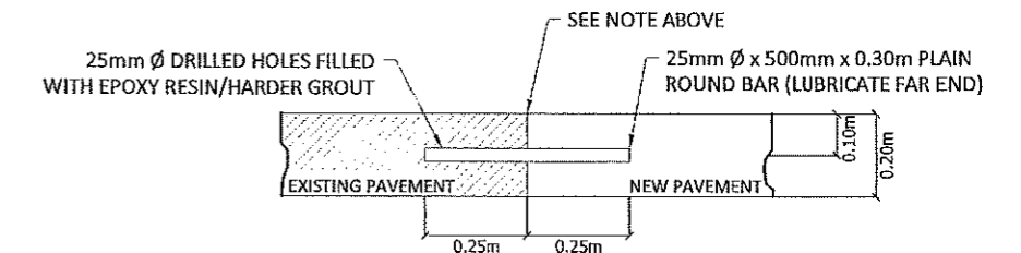
CONSTRUCTION JOINT SCALE: 1:20m
