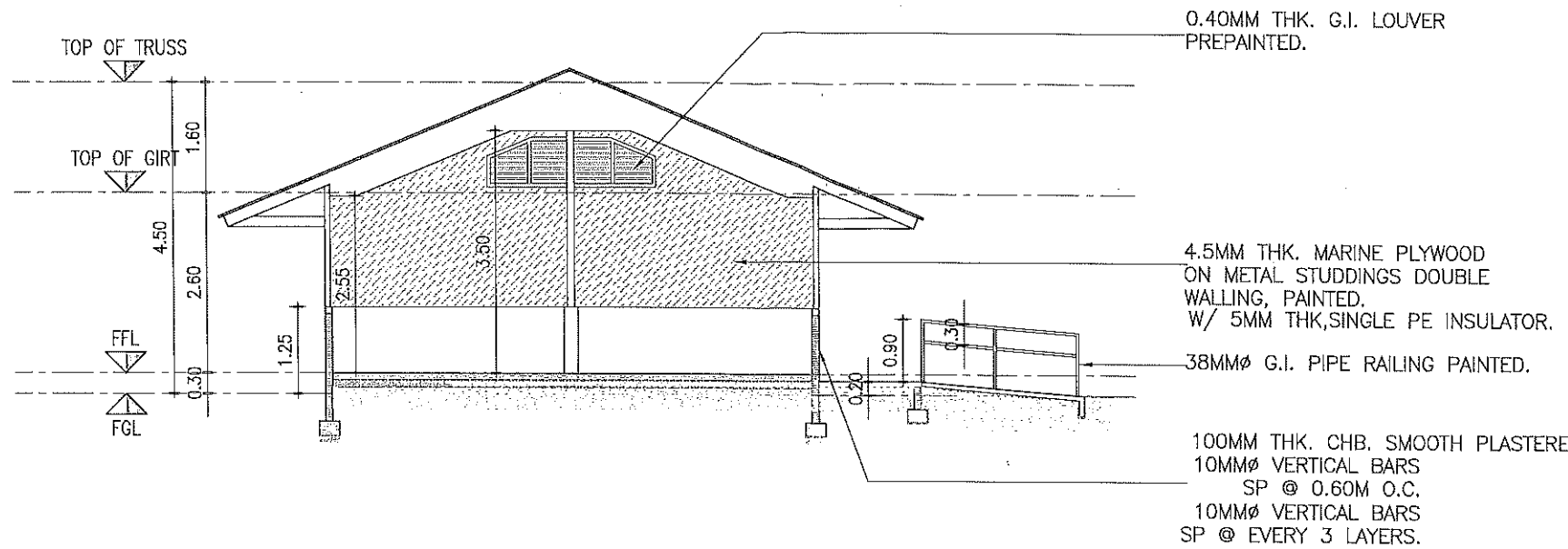
2 CROSS SECTION A-4 SCALE 1:100 M.
