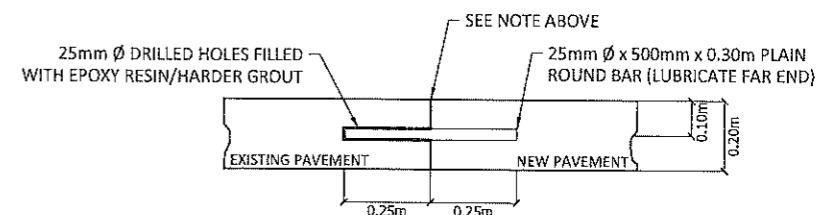
CONSTRUCTION JOINT SCALE: 1:20m
