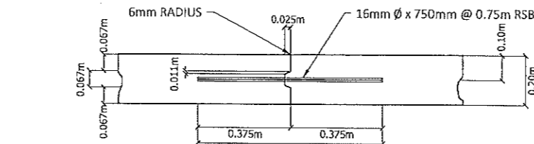
LONGITUDINAL CONST. JOINT TO BE USED FOR HALF WIDTH OR LANE AT TIME OF CONSTRUCTION SCALE: 1:20m
