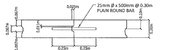
KEYED TRANSVERSE CONST. JOINT TO BE PLACED ONLY IN MIDDLE THIRD OF NORMAL JOINT INTERVAL SCALE: 1:20m
