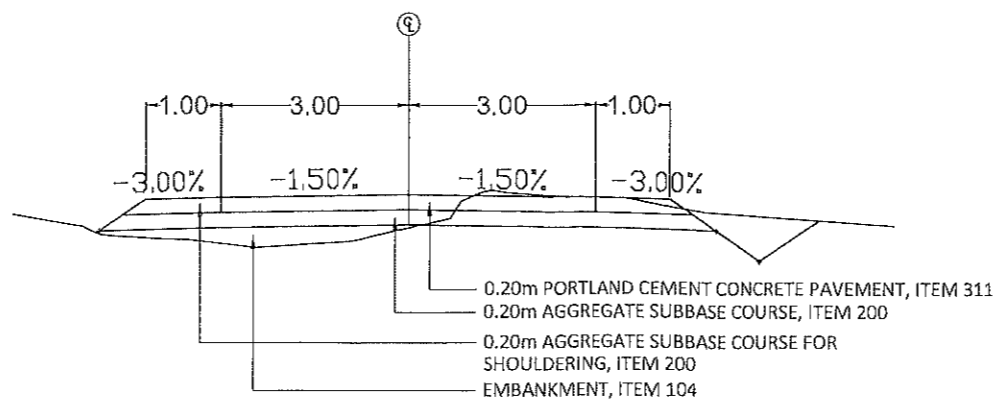
TYPICAL THRU CUT AND FILL SECTION
