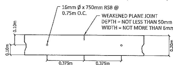
WEAKENED PLANE JOINT SCALE: 1:20m
