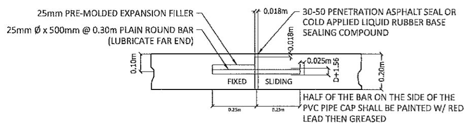
TYPICAL EXPANSION JOINT TO BE PLACED EVERY 36.00 M. O.C. SCALE: 1:20m
