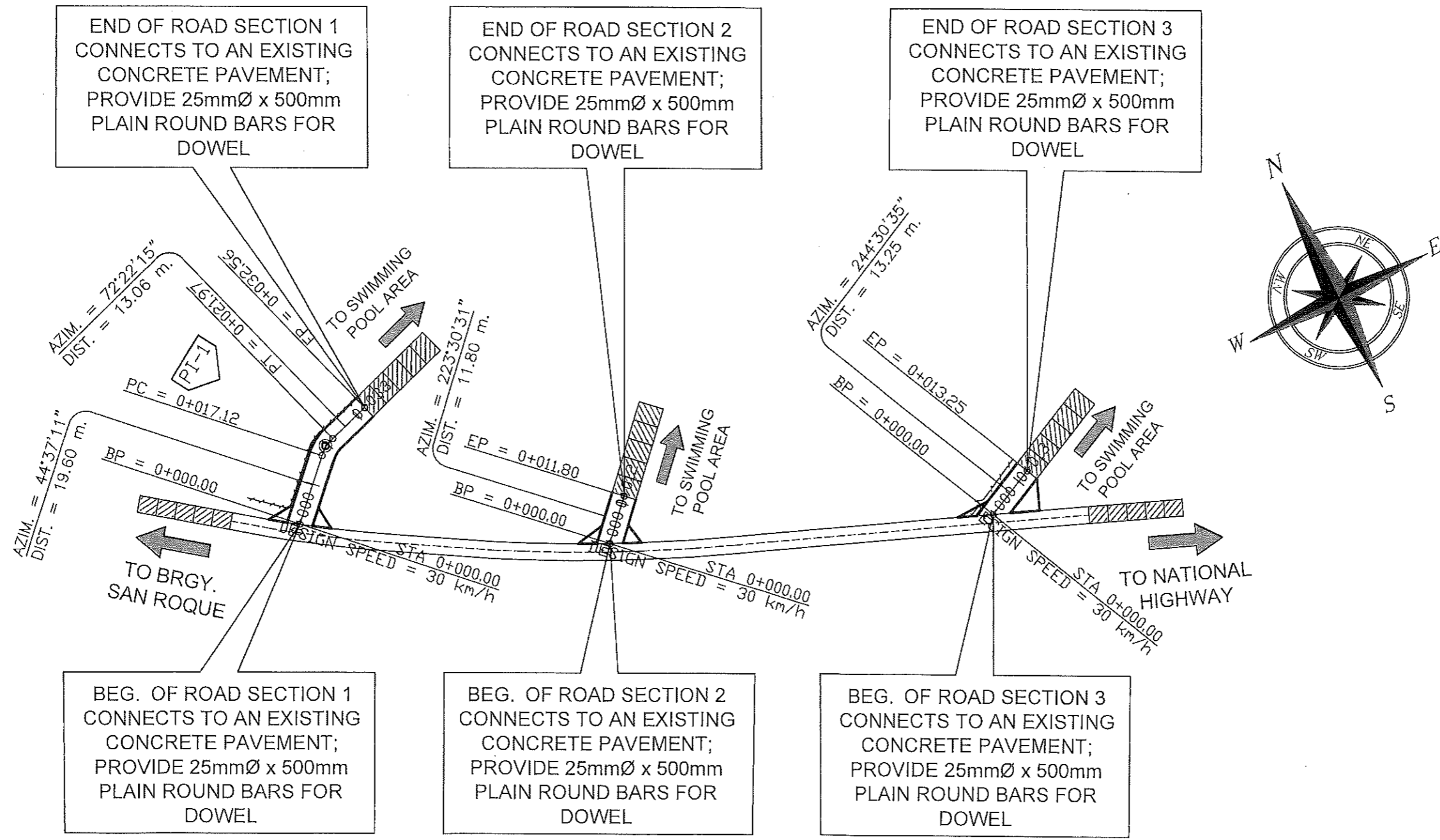
GENERAL PLAN SCALE DNTS
