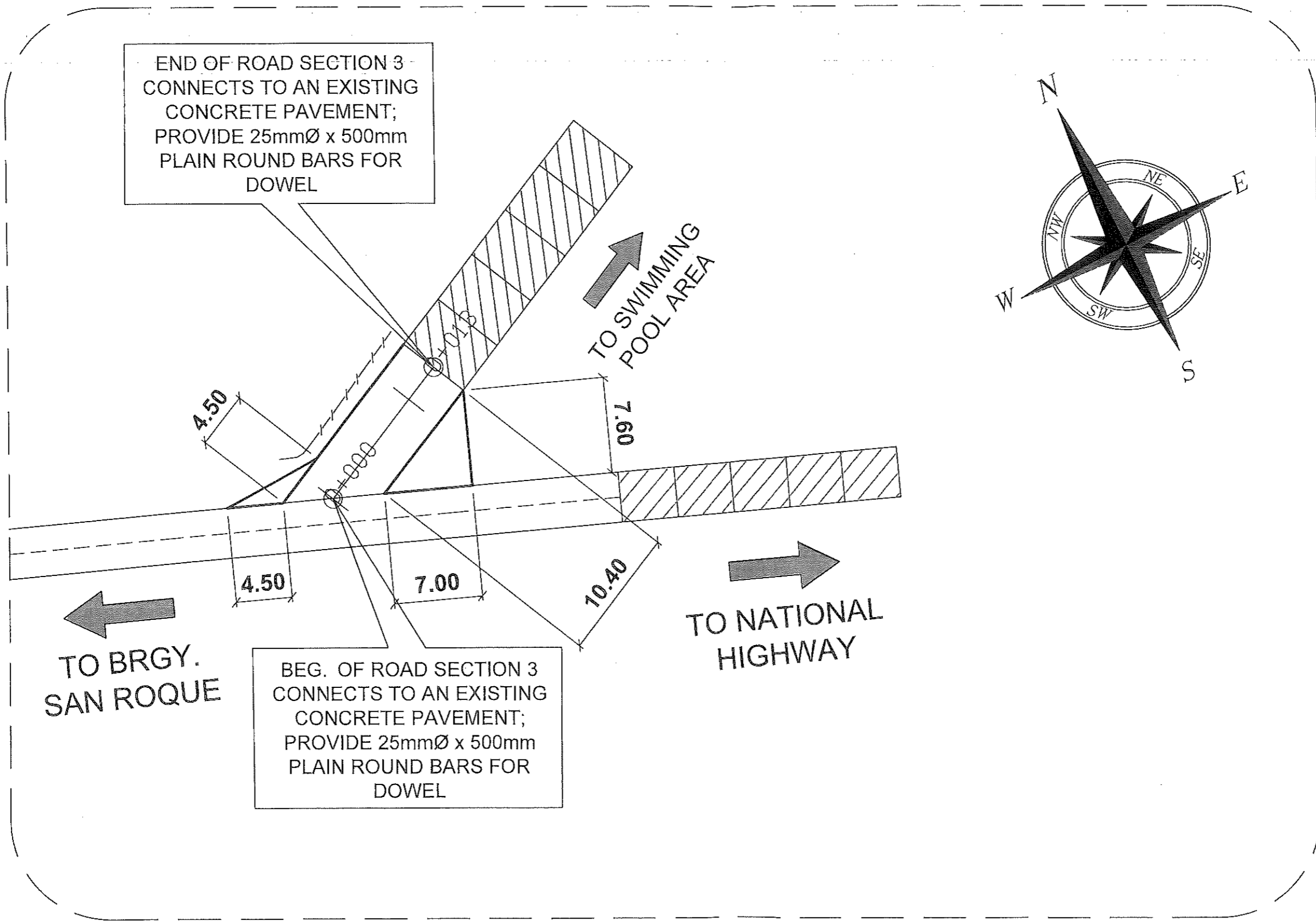
ROAD SECTION 3 FLARE DETAILS SCALE DNTS
