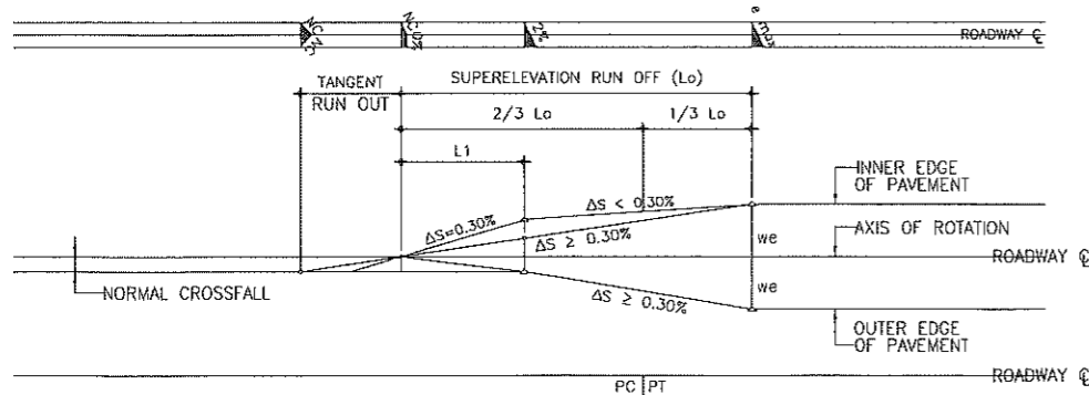
TRANSITION: CIRCULAR CURVE - STRAIGHT - CIRCULAR CURVE CASE 2
