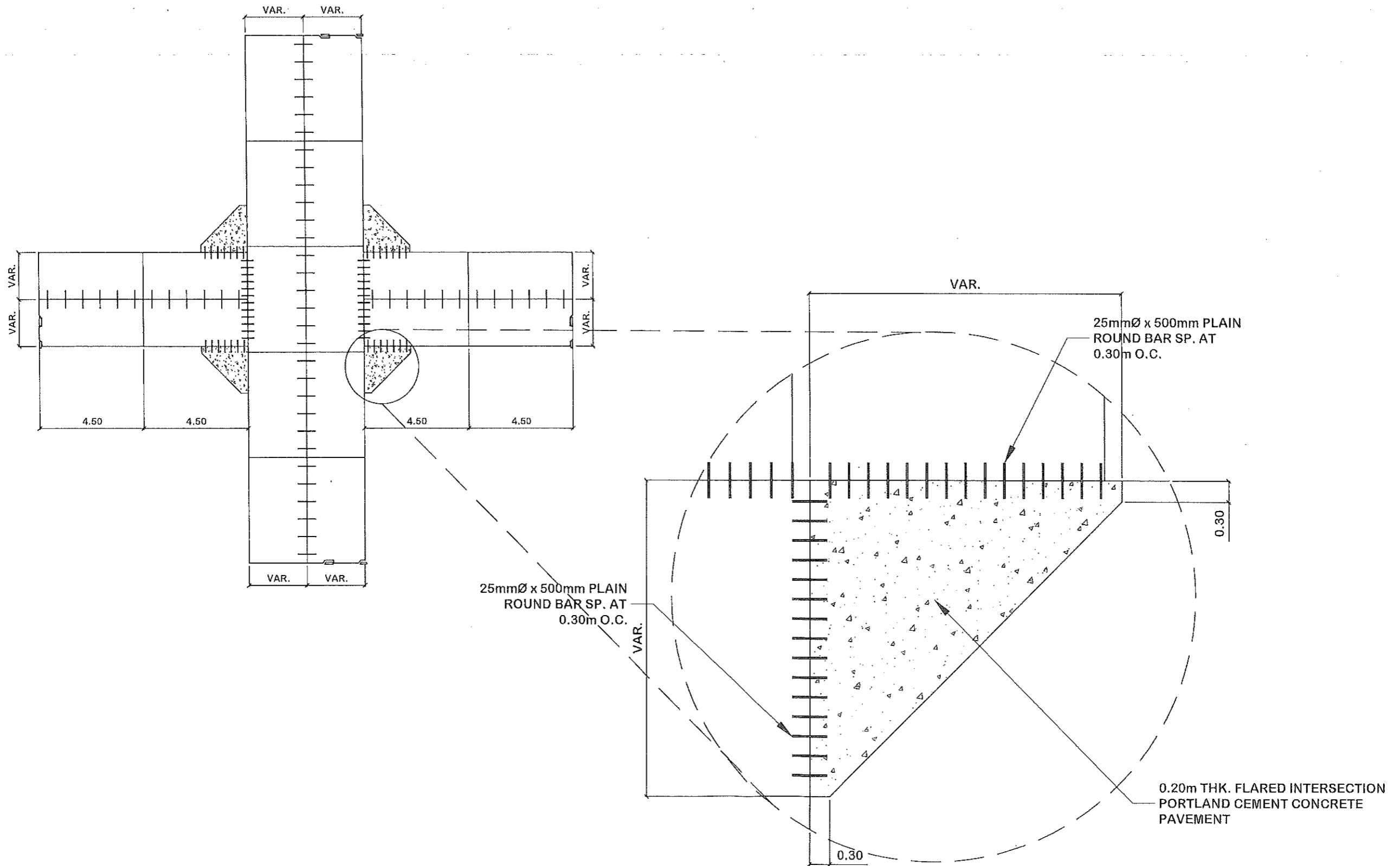
TYPICAL FLARED INTERSECTION DETAIL SCALE DNTS
