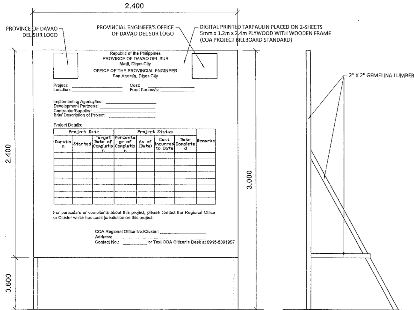
PROJECT BILLBOARD (COA STANDARD) SCALE DNTS
