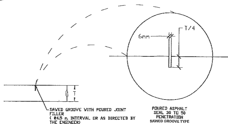
WEAKENED PLANE JOINT OR CONSTRUCTION JOINT NOT TO SCALE
