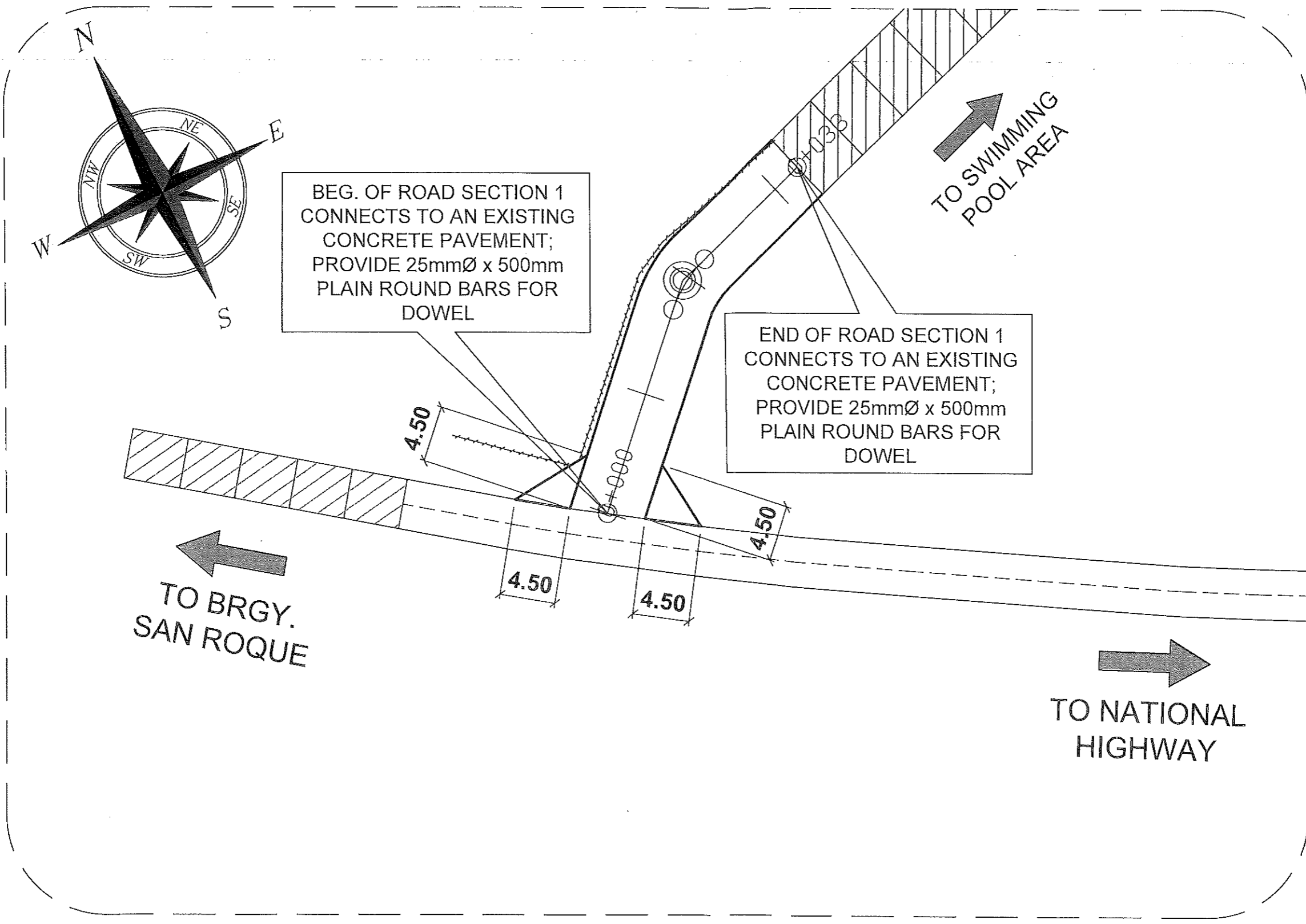
ROAD SECTION 1 FLARE DETAILS SCALE DNTS
