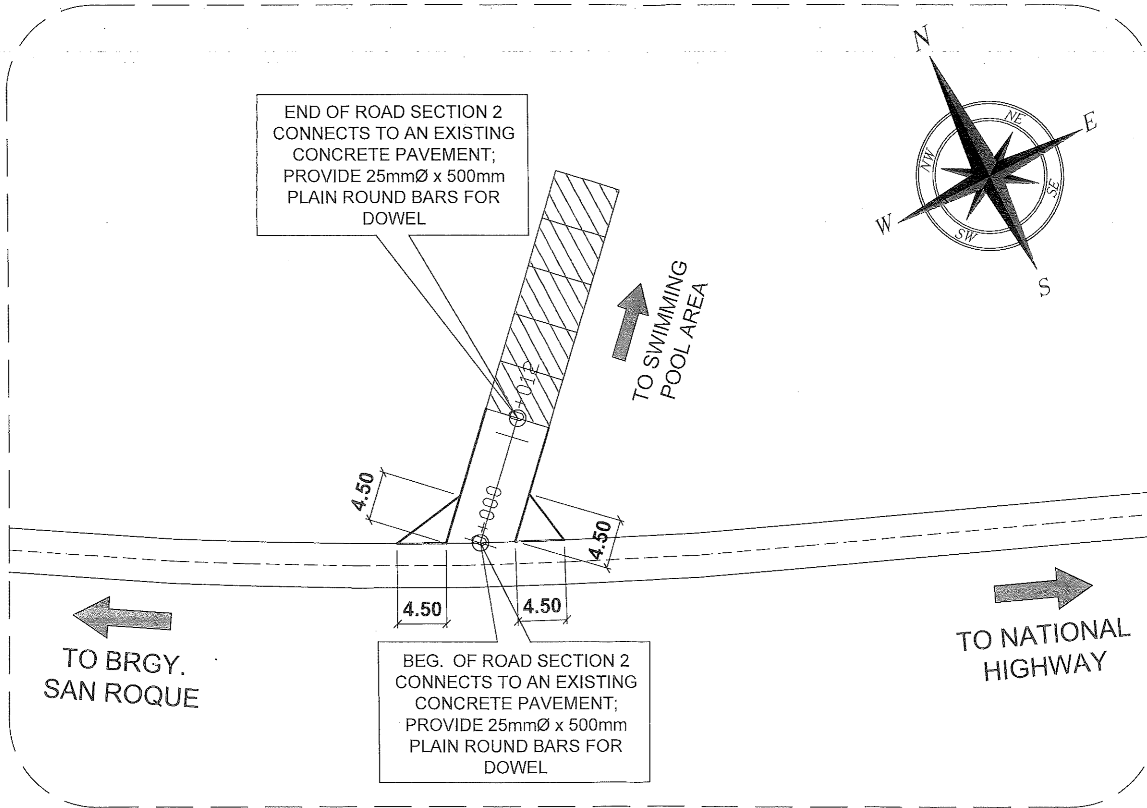
ROAD SECTION 2 FLARE DETAILS SCALE DNTS
