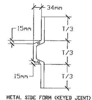
DETAIL OF SIDE FORMS NOT TO SCALE
