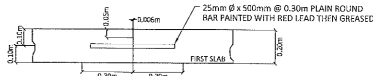
BUTT TRANSVERSE CONSTRUCTION OR CONTRACT JOINT SCALE: 1:20m
