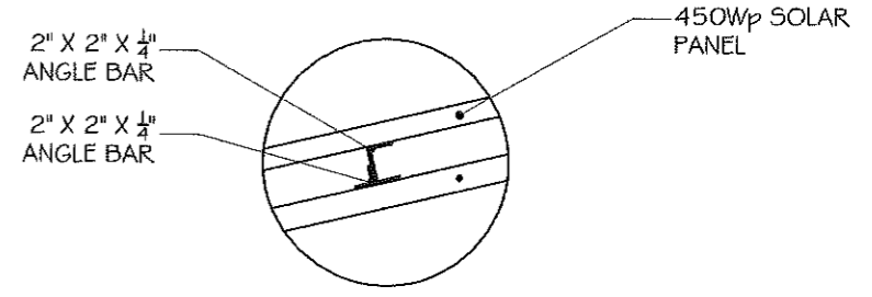
DETAILS 'A'
