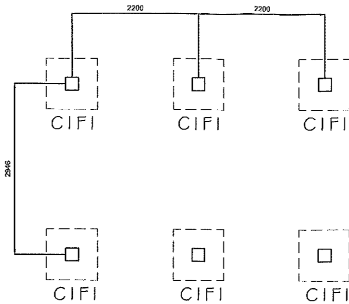
FOUNDATION PLAN
